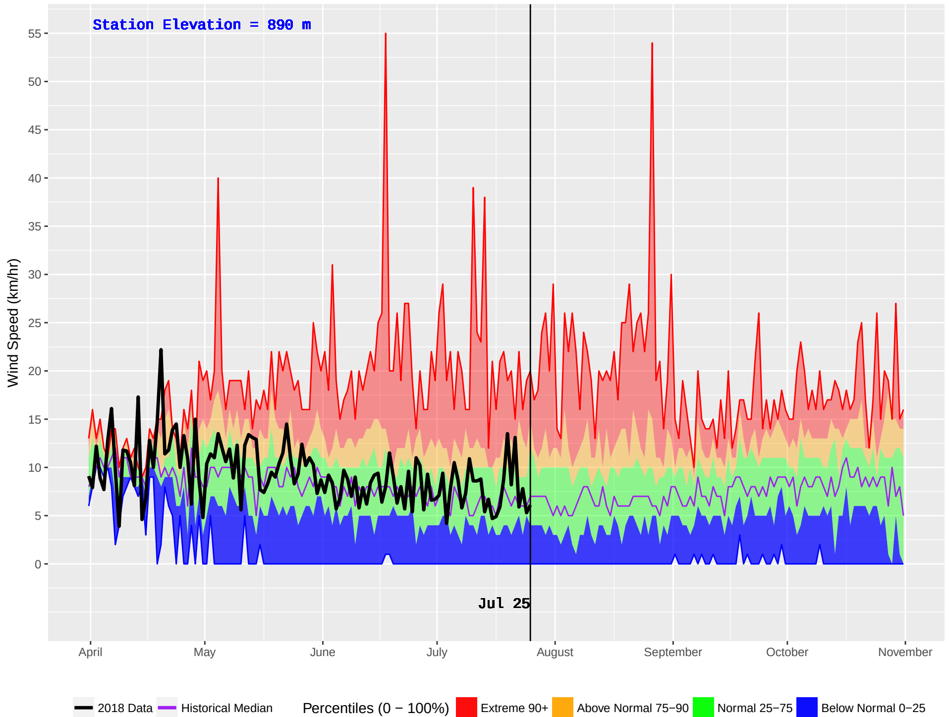
ISKUT (112) : Historical (1979–2016) and Current (2018) Noon Wind Speed
