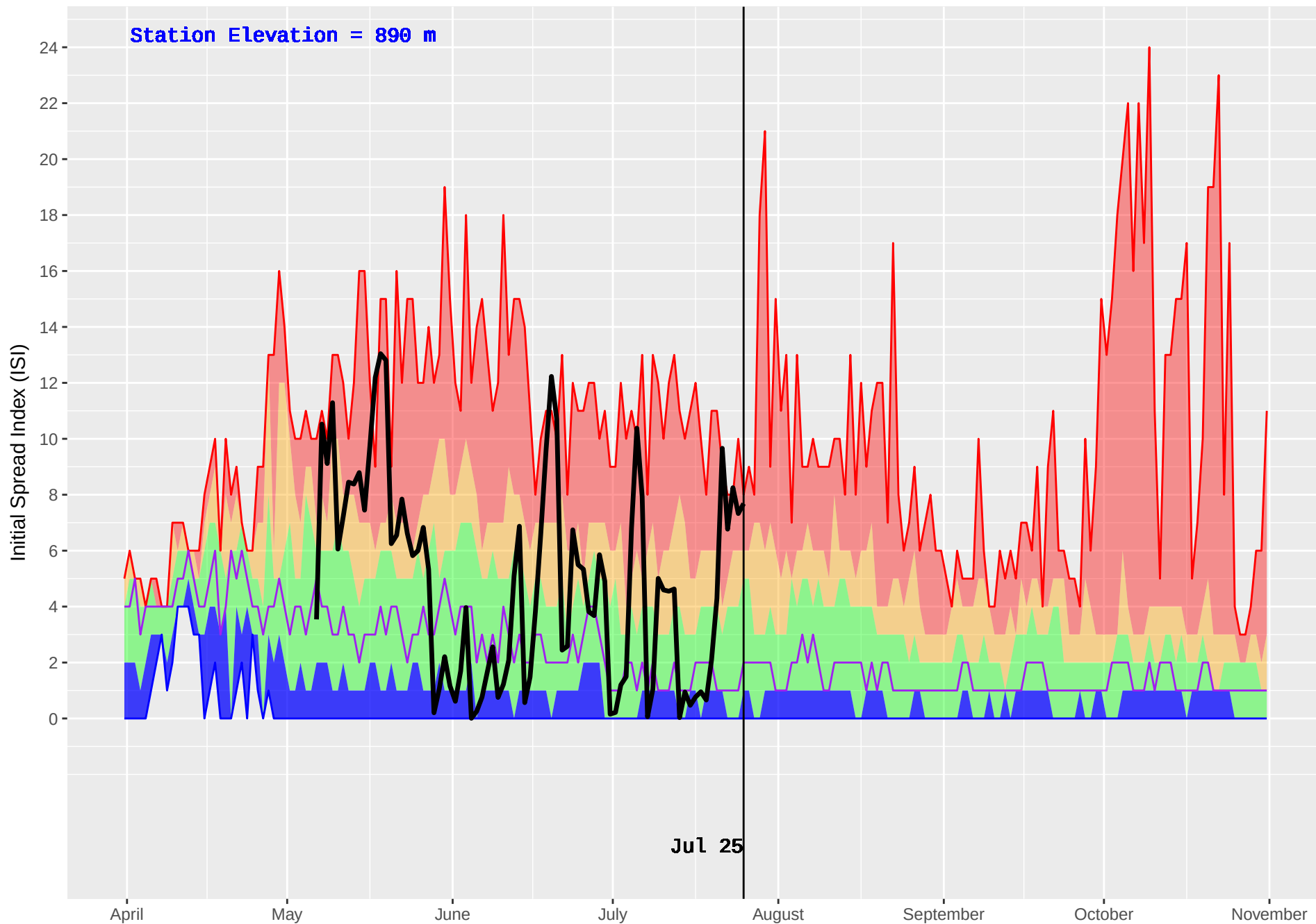
ISKUT (112) : Historical (1979–2016) and Current (2018) Noon Initial Spread Index (ISI)
