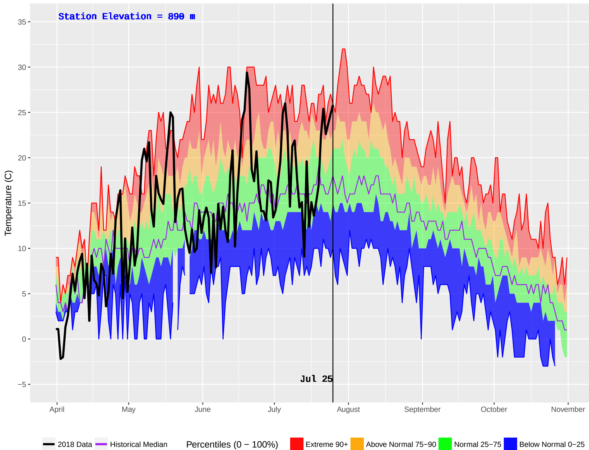
ISKUT (112) : Historical (1979–2016) and Current (2018) Noon Temperature
