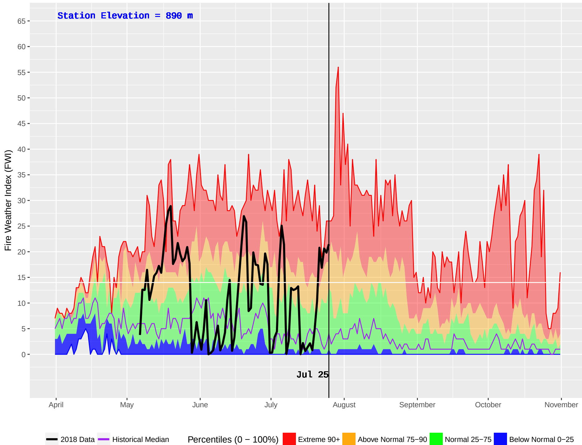
ISKUT (112) : Historical (1979–2016) and Current (2018) Noon Fire Weather Index (FWI)
