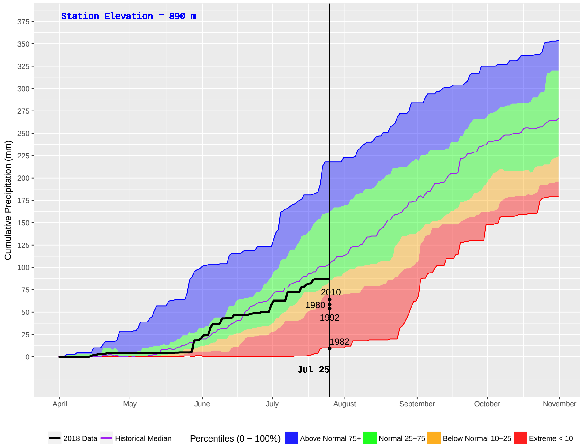
ISKUT (112) : Historical (1979–2016) and Current (2018) Noon Cumulative Precipitation
