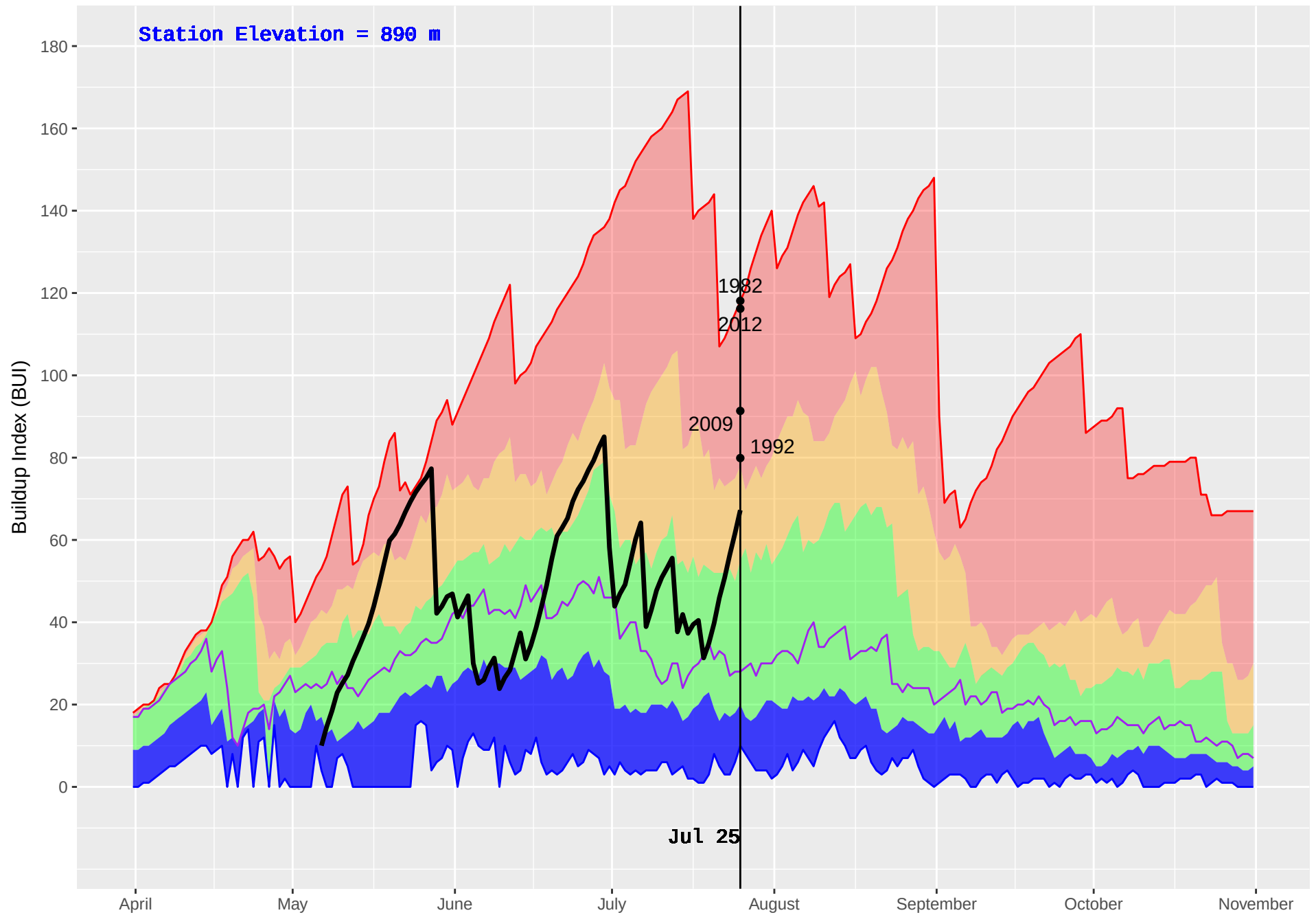
ISKUT (112) : Historical (1979–2016) and Current (2018) Noon Buildup Index (BUI)
