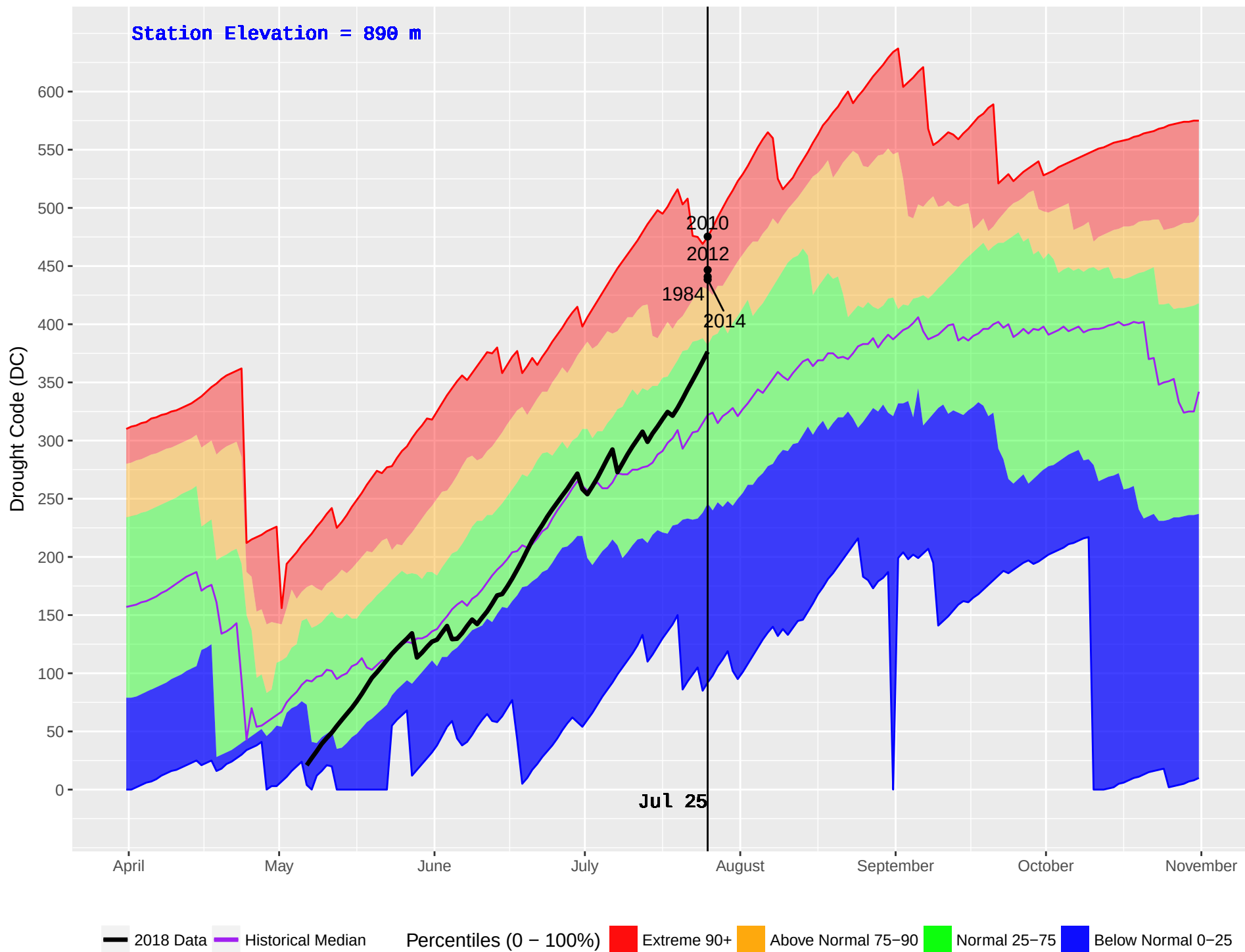
ISKUT (112) : Historical (1979–2016) and Current (2018) Noon Drought Code (DC)
